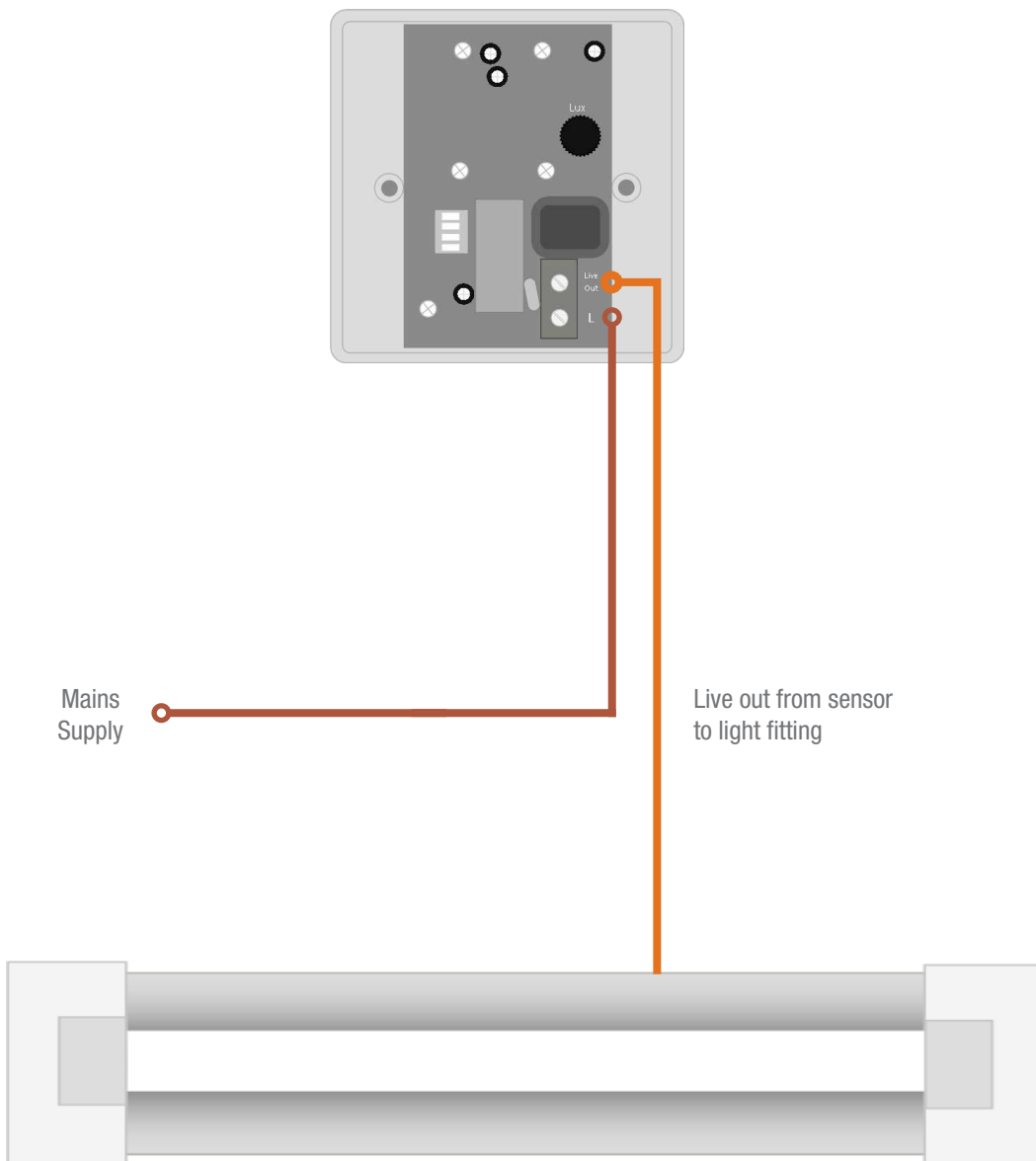
Rear view of Sensor
