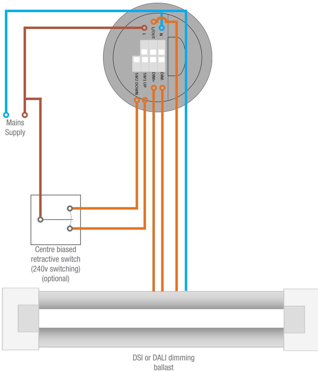
Rear view of Sensor
