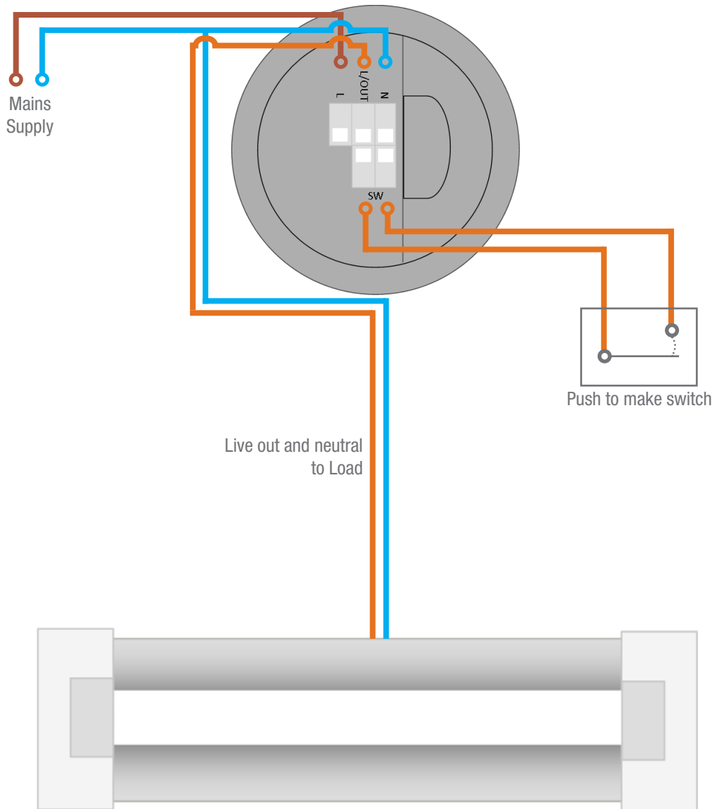
Rear view of sensor
