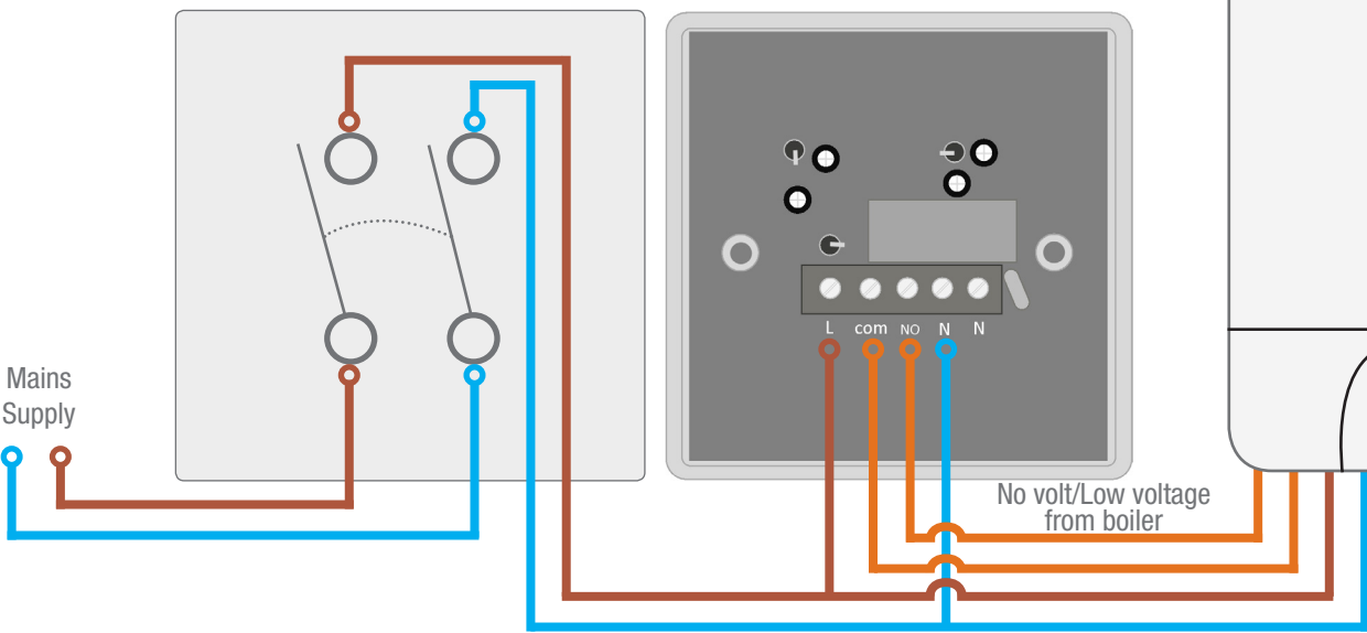
Switched fused spur
