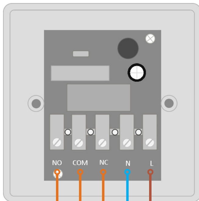
Rear of the unit
