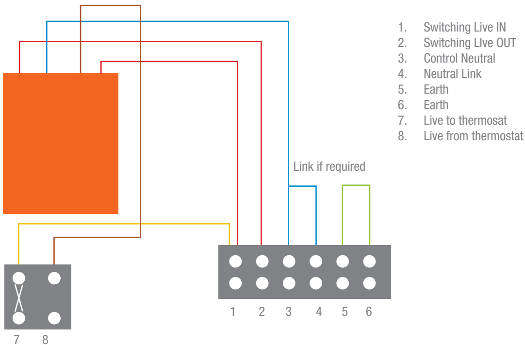
PRE9030F Relay Module schematic wiring diagram
