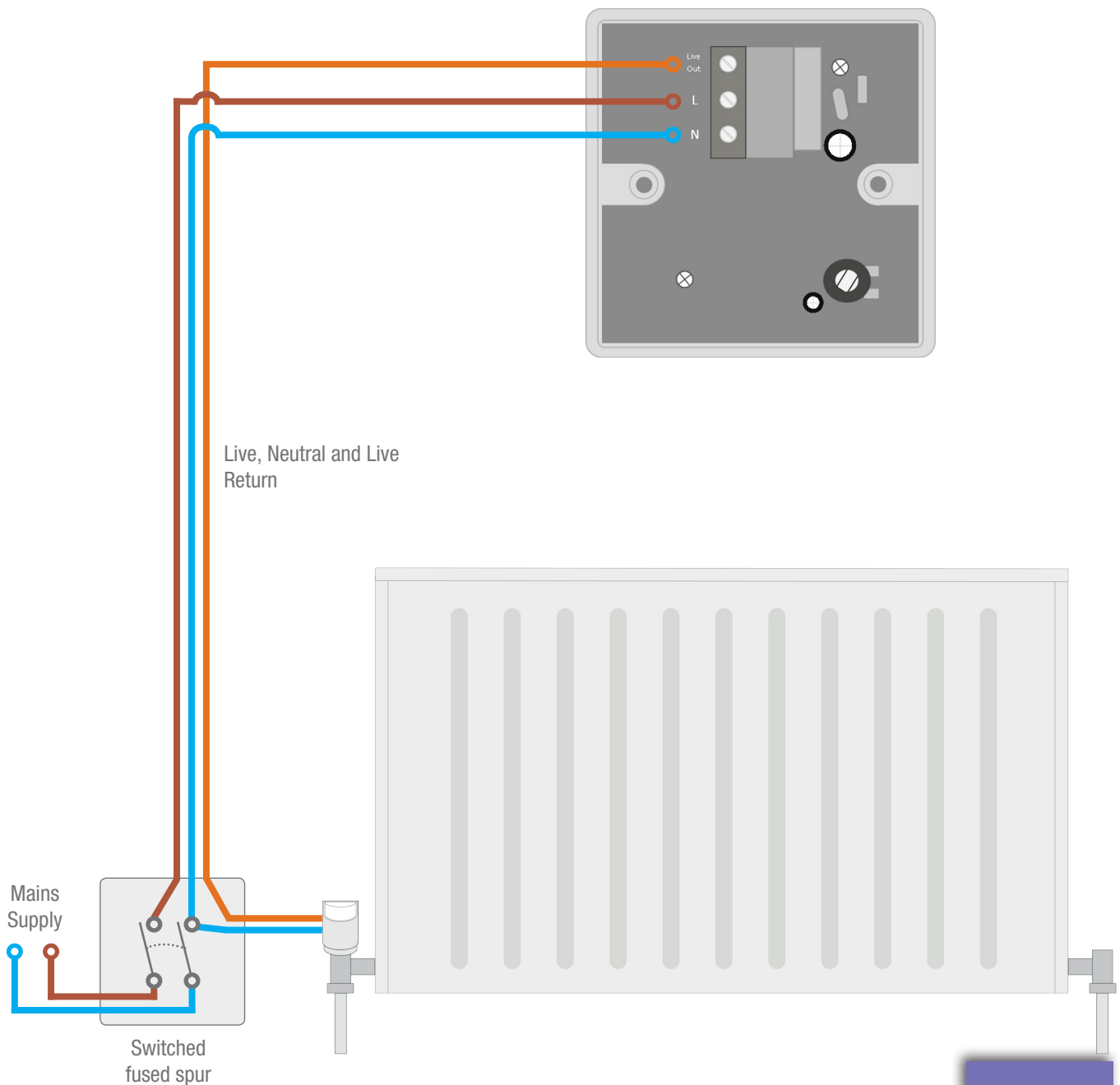
Rear view of a 5 series thermostat
