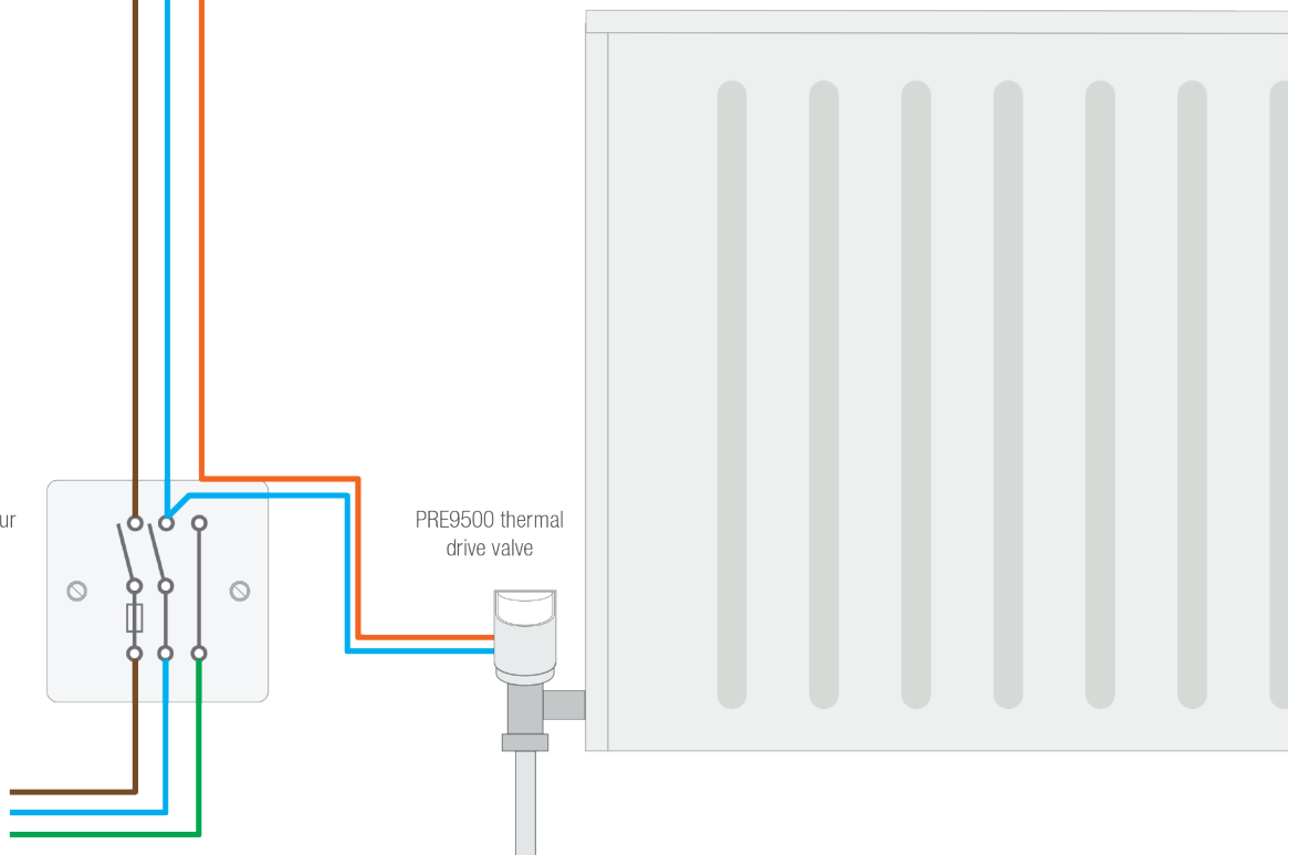
Mains supply
